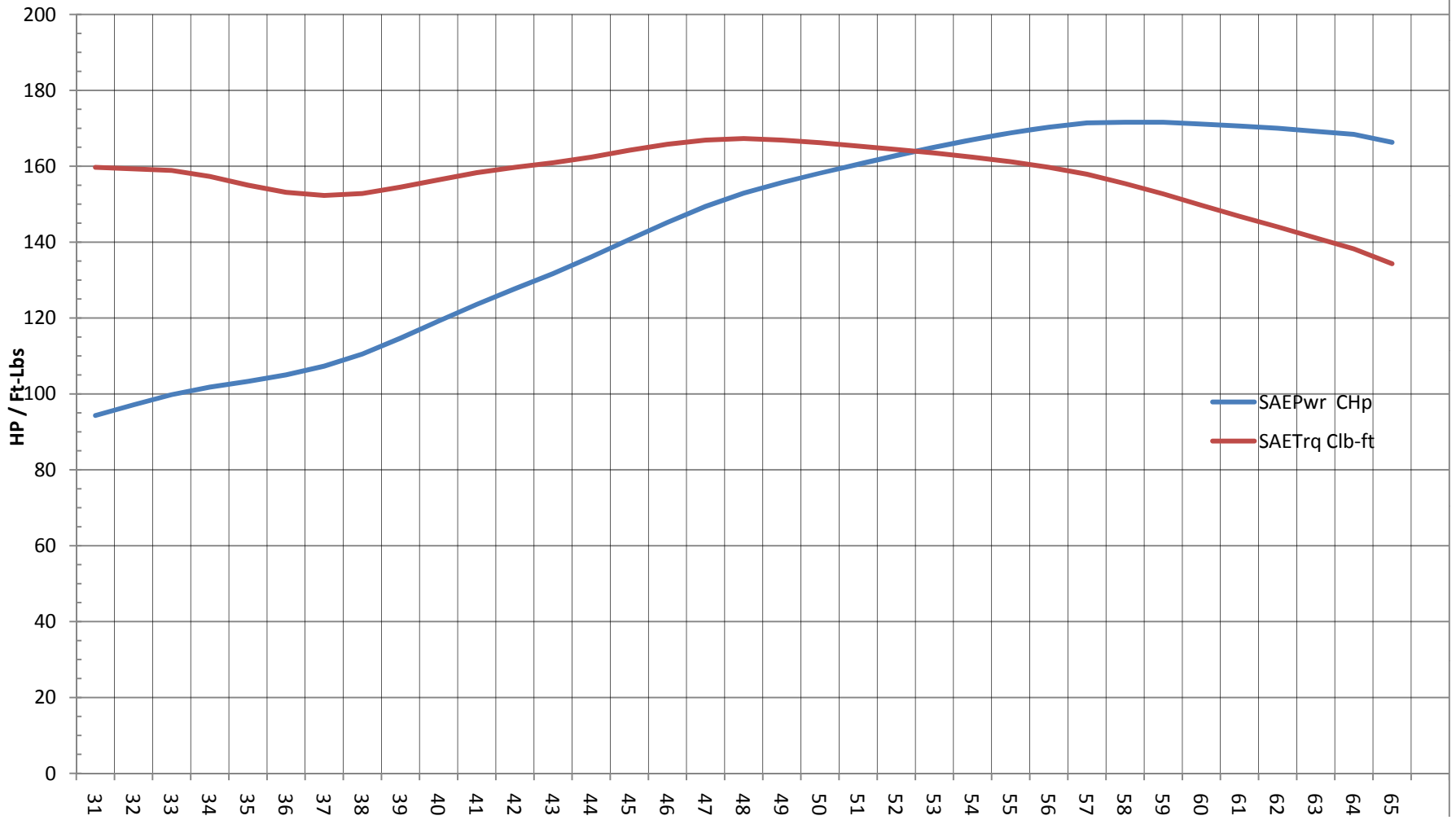
Typical FE Power and Torque
