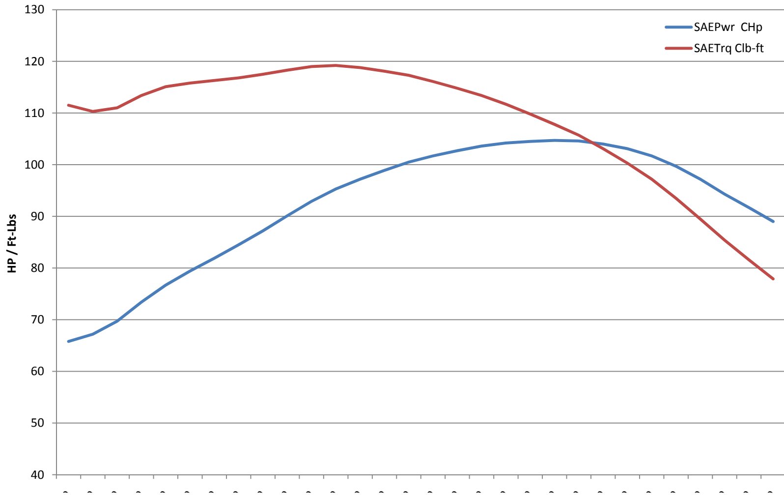
SRF Engine HP / Torque
